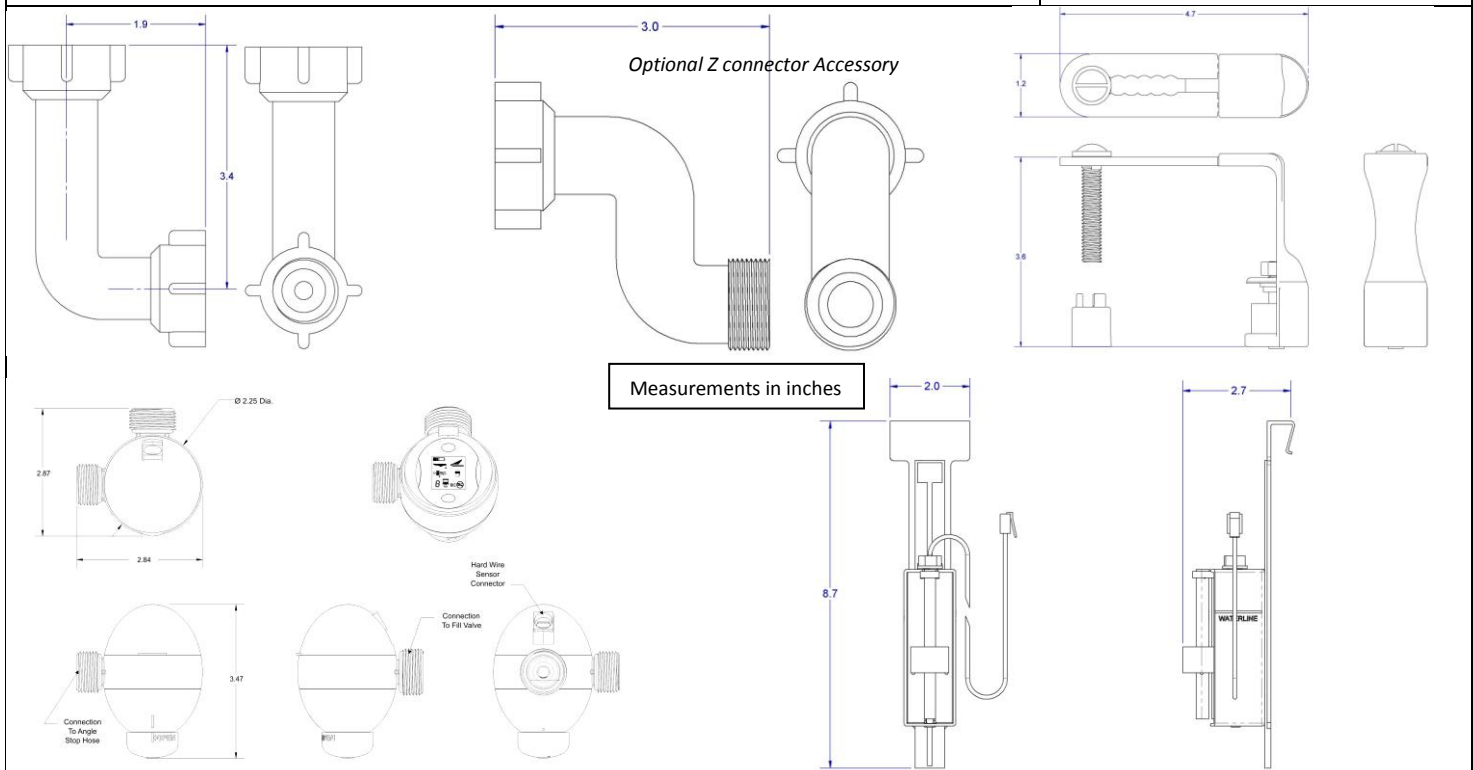
TG 1000 Complete Installation With Bowl Overflow Elimination and Water Conservation sensors
